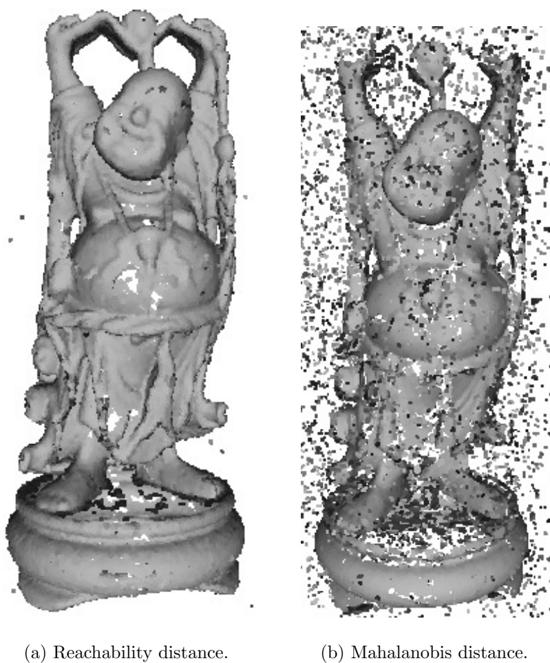
Figure 5.5: Buddha, filtered. The reachability distance-based filtering method leaves almost no outliers.
